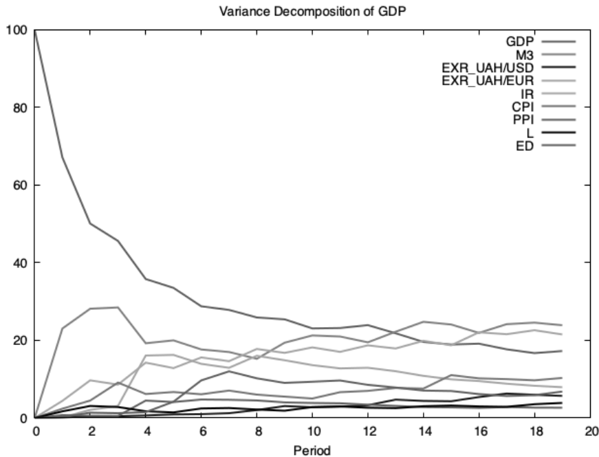
Figure 3 Variance decomposition
